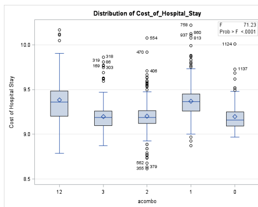
Figure 4.3 Distribution of Cost by Acombo (Natural Log of Cost)
