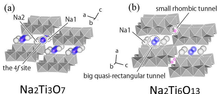
Figure 7. Schematic structure of \text{Na}_2\text{Ti}_3\text{O}_7 and \text{Na}_2\text{Ti}_6\text{O}_{13} . Large blue and small red spheres represent the additional \text{Na}^+ and \text{Li}^+ , respectively.
