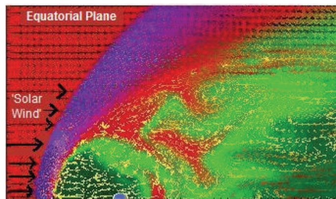
Figure 1. Earth's Bow Shock. Magnetohydrodynamic (MHD) turbulence vectors. Note the implied but unrecognised speed change we identify at the shock crossing. (NASA)
